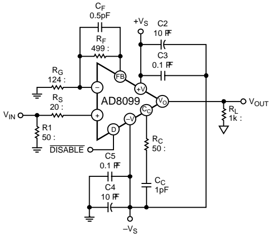
Figure 64. Amplifier Configuration for CSP and SOIC Packages, Gain = +5
