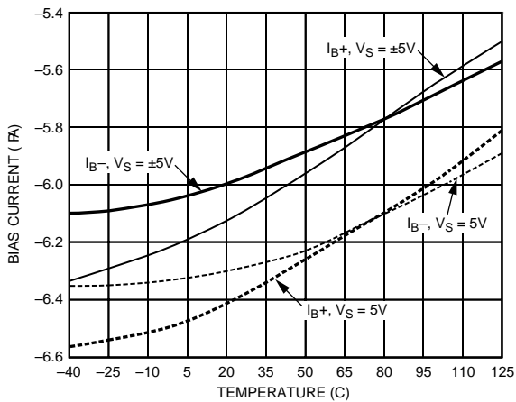
Figure 54. Input Bias Current vs. Temperature (DISABLEn Floating)
