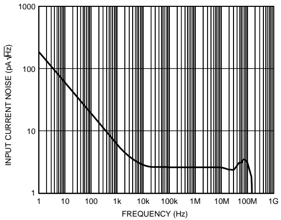
Figure 48. Input Current Noise vs. Frequency (DISABE = Open)
