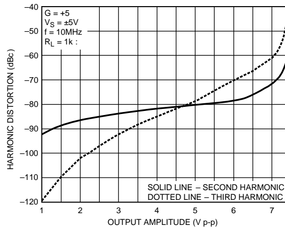
Figure 34. Harmonic Distortion vs Output Amplitude (CSF)
