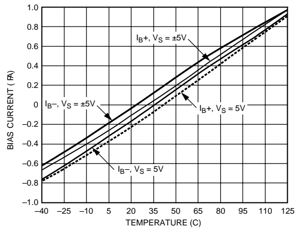
Figure 57. Input Bias Current vs. Temperature (DISABLEn = +V_S)
