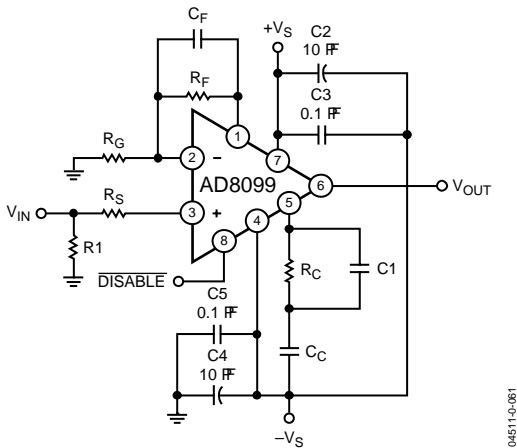
Figure 59. Wideband Noninverting Gain Configuration (SIO)
