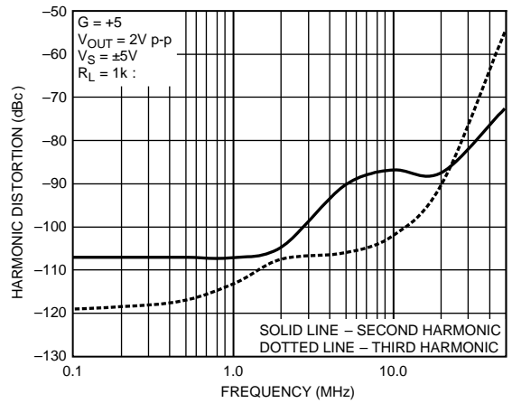
Figure 26. Harmonic Distortion vs Frequency (CSF)
