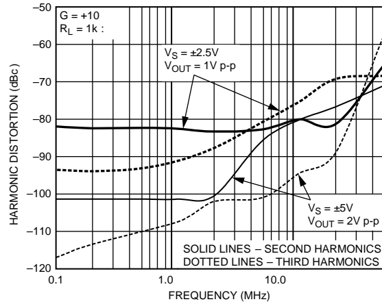
Figure 32. Harmonic Distortion vs Frequency for Various Supplies (CSF)
