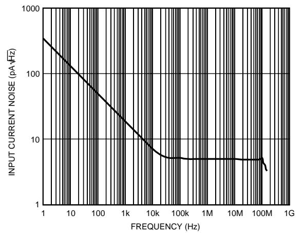
Figure 51. Input Current Noise vs. Frequency (DISABE = +Vs)
