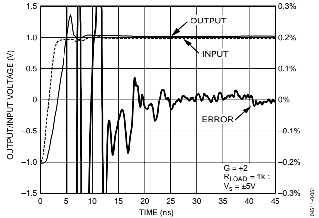
Figure 45. Shot Term Settling Time (SOIC)
