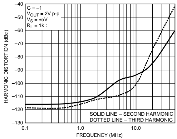
Figure 28. Harmonic Distortion vs Frequency (CSF)
