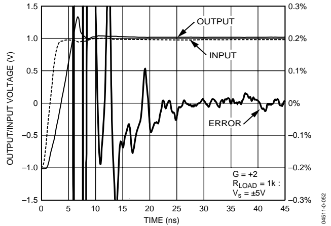
Figure 44. Shot Term Settling Time (CSP)
