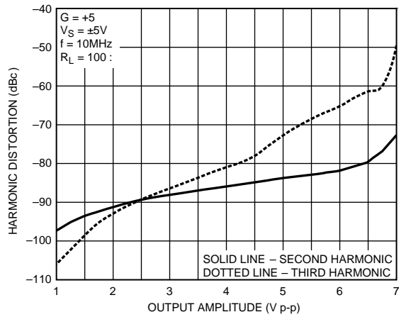
Figure 33. Harmonic Distortion vs Output Amplitude (CSF)
