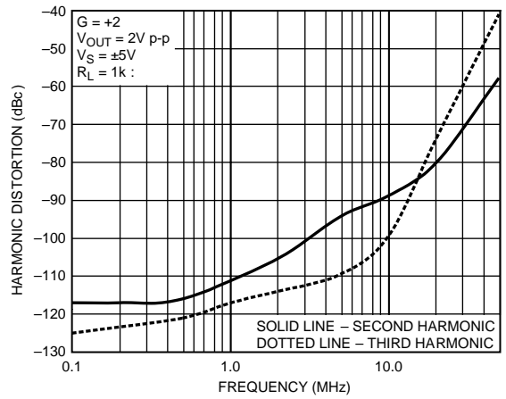
Figure 27. Harmonic Distortion vs Frequency (CSF)
